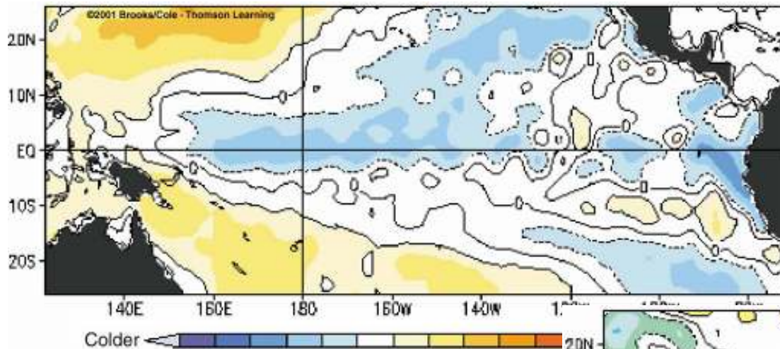
Fig. 7.27: (a) upwelling along equator and S. Amer. Coast keeps water cool
