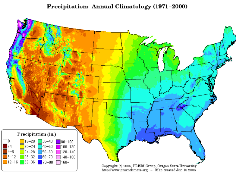
Figure 2. Average precipitation (in inches) across the conterminous United States, as modeled from 1971-2000 NOAA Cooperative Station normals and NRCS SNOTEL data. Image from http://www.prismclimate.org
