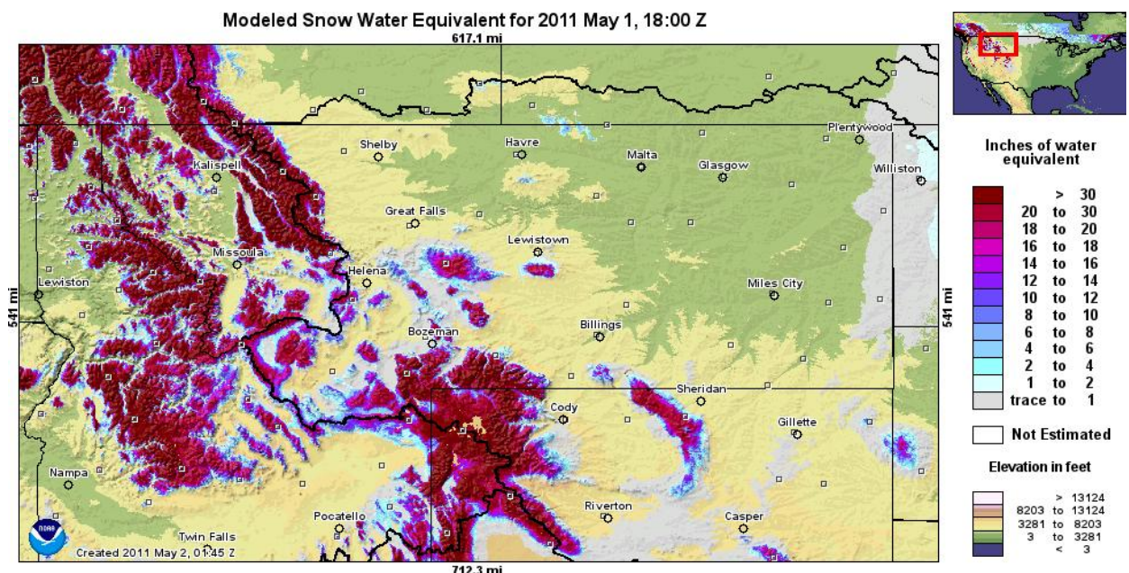
Figure 14. Modeled snow water equivalent for May 1, 2011. Image courtesy of NOHRSC.
