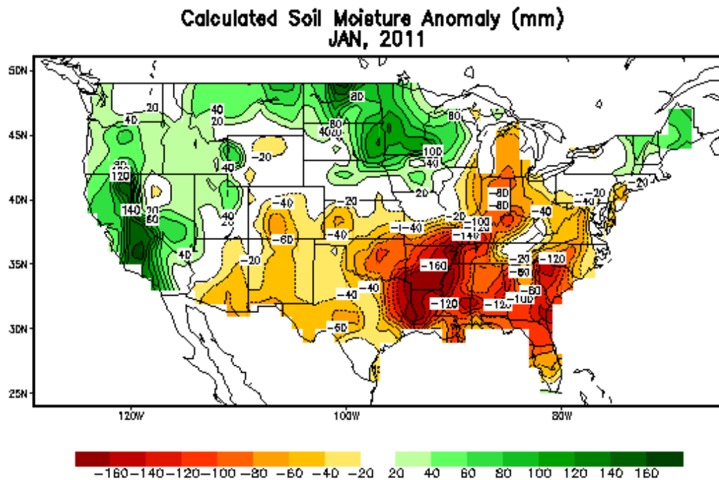
Figure 11. Calculated soil moisture anomaly as of January 2011 (in millimeters). Data from NOAA at http://www.cpc.ncep.noaa.gov/soilmst/index_jh.html
