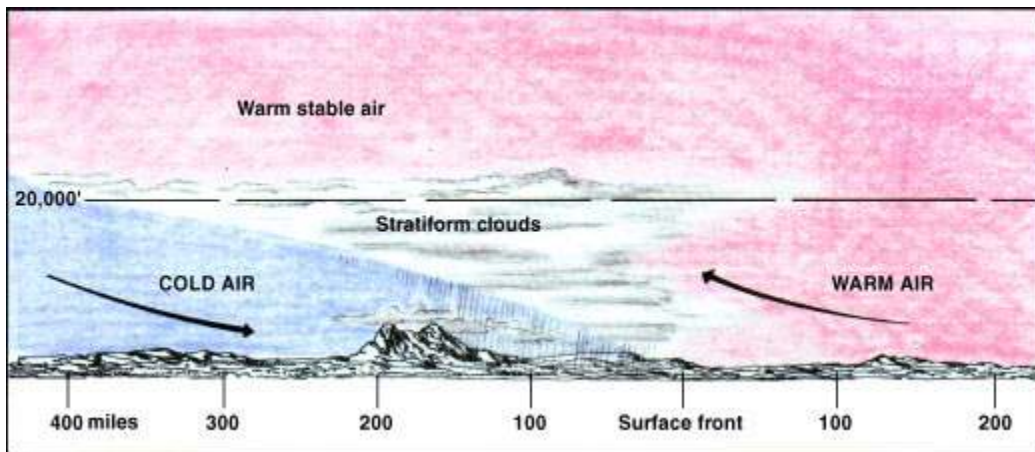
Figure 1-3. Post-frontal Fog Associated with Slow-Moving Cold Fronts. Persistent fog may occur with this type of cold front.
